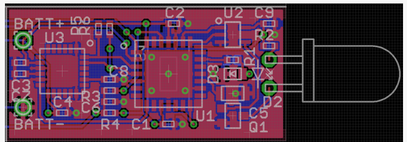
Emitter board
