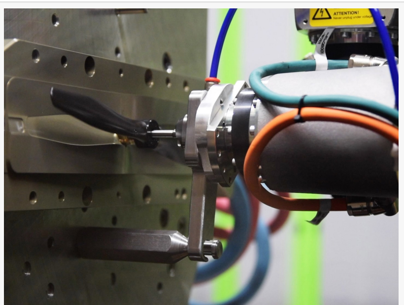
Master Airscrew propeller manufacturing
