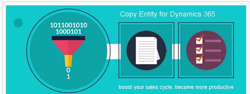
Dynamics 365 CopyEntity
