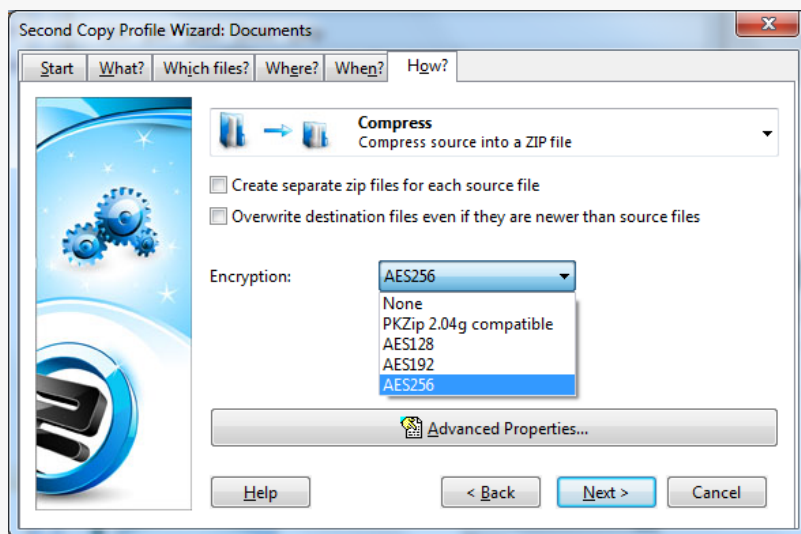
Second Copy compression and encryption
