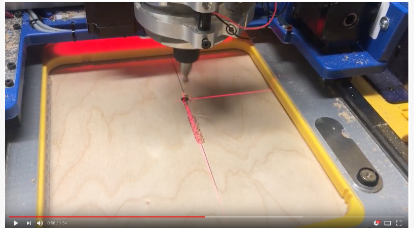
Handibot, the portable CNC, cutting Lockdowel insertion holes.
