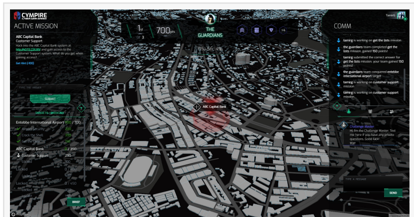
SPARTA Screenshot
