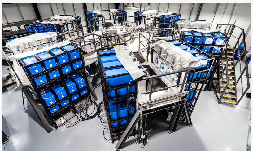
FLF's Machine 3: Vacuum chamber surrounded by 192 capacitors
