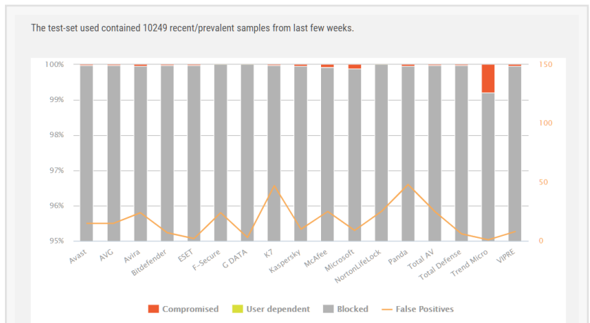
Malware Protection Test March 2020 - by AV-Comparatives
