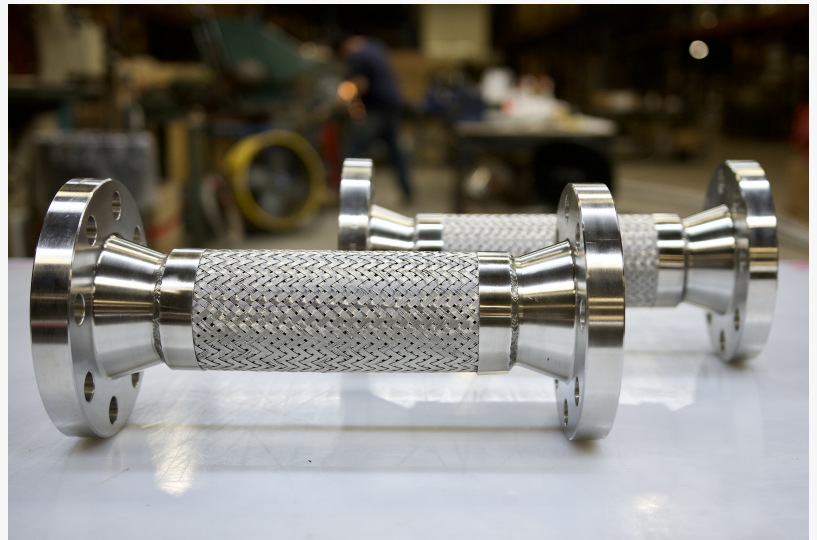
Penflex 3-Inch Inconel Assemblies
