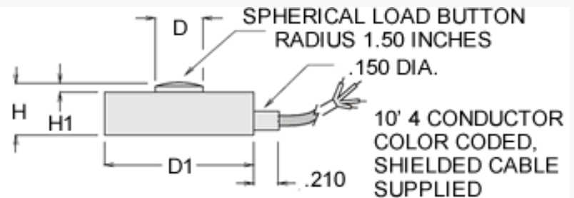
SLB Series Load Cell Specifications
