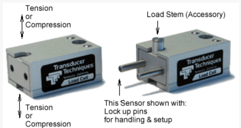
GSO Series Precision Gram Load Cell
