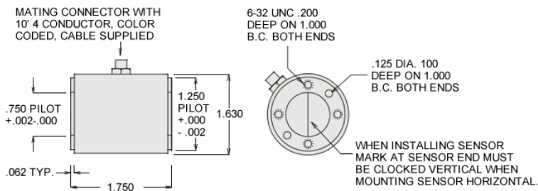
RTS Series Reaction Torque Sensor Specifications
