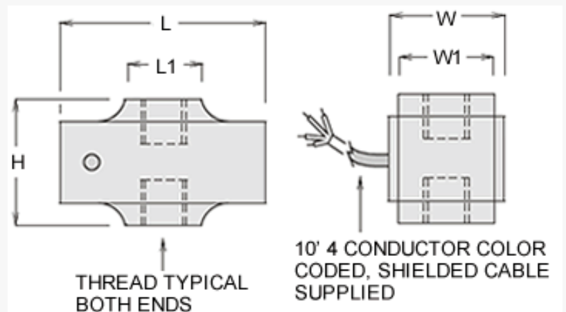
MLP Series Mini Low Profile Load Cell Specifications
