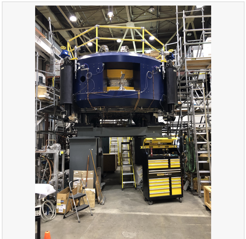
Best 70 MeV Cyclotron Magnet Assembly
