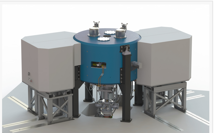
Best 6–15 MeV Compact Variable Energy Cyclotron System (Closed View with Shielding)
