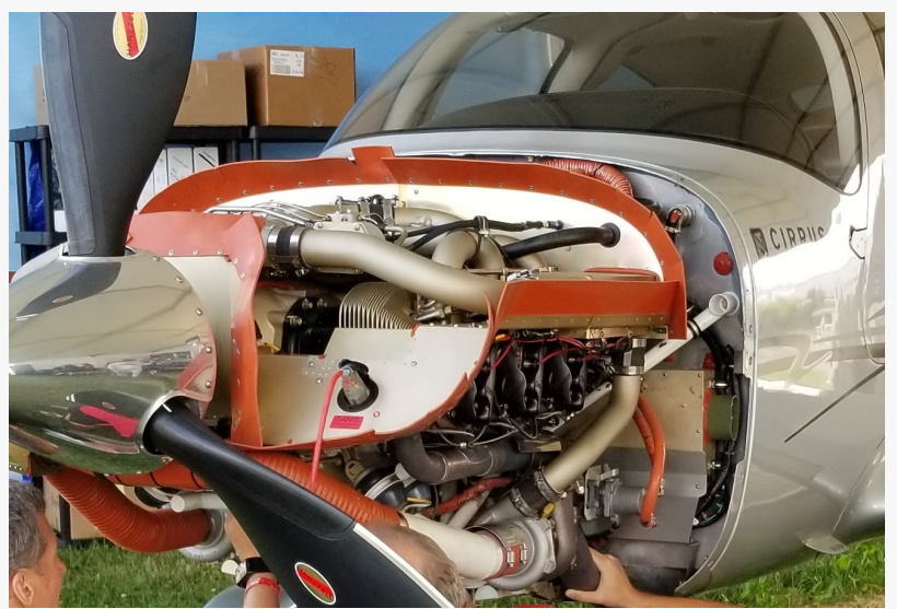
Tanis preheat system for Cirrus SR-22
