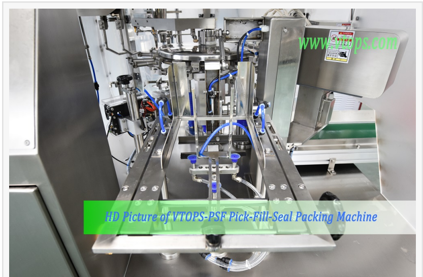
Pouch Loading Device of Pick Fill Seal Packaging Machine
