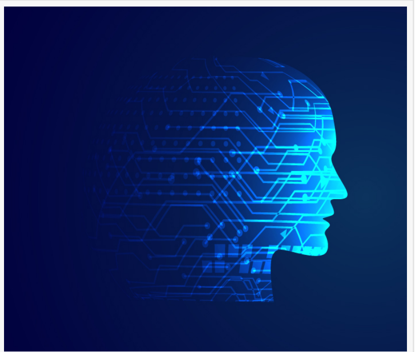
Cryptography DNA
