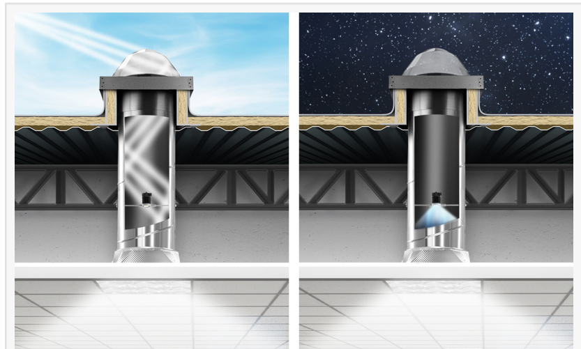
The Solatube Integrated LED Light Kit
