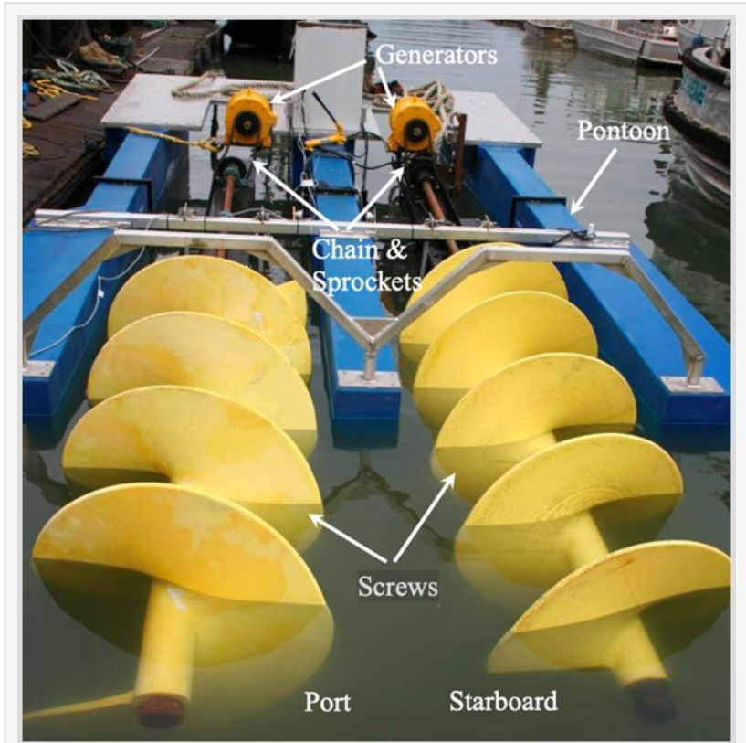
Open water test unit
