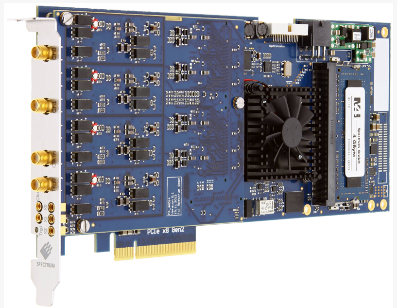
Spectrum M4i.4450-x8 2-channel digitizer with 500 MS/s speed
