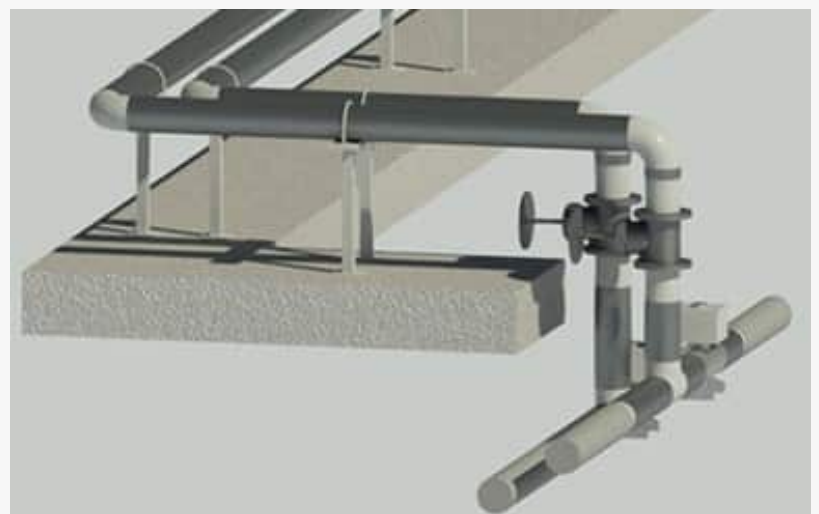
Mechanical Piping Model for Pollution Control Plant in Lorton, VA
