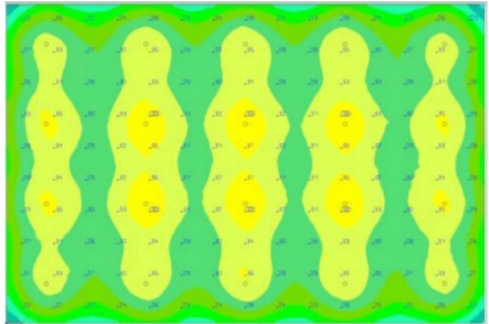
80 x 120 Indoor Arena Lighting with 20 SYMA
