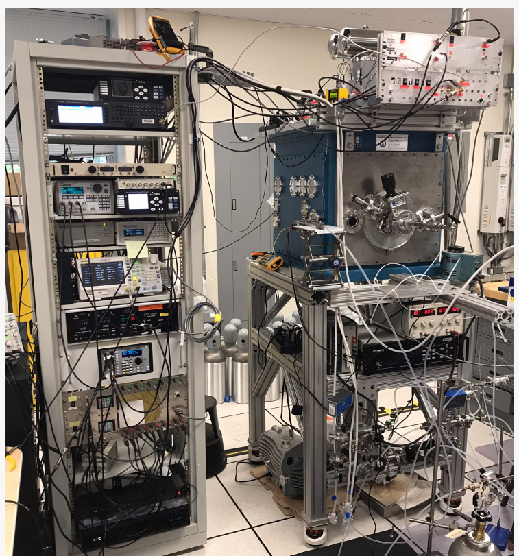
A groundbreaking step forward: The new developed microwave spectrometer at the Harvard Smithsonian Center for Astrophysics
