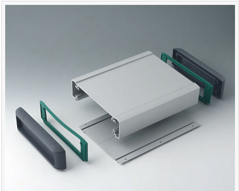
SMART-TERMINAL extruded aluminum enclosures with plastic end panels and TPV sealing gaskets.
