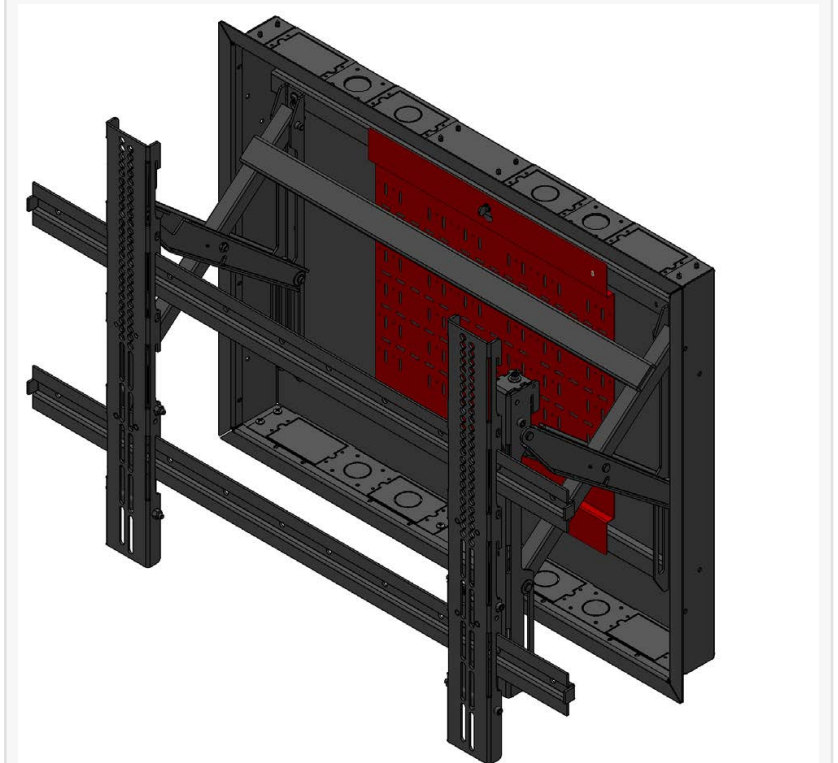
Wallmate Slim In-Wall Mounting System For 2.5" Stud Walls Helps Achieve ADA Compliance With Displays Larger Than 55" And Up To 225 lbs.
