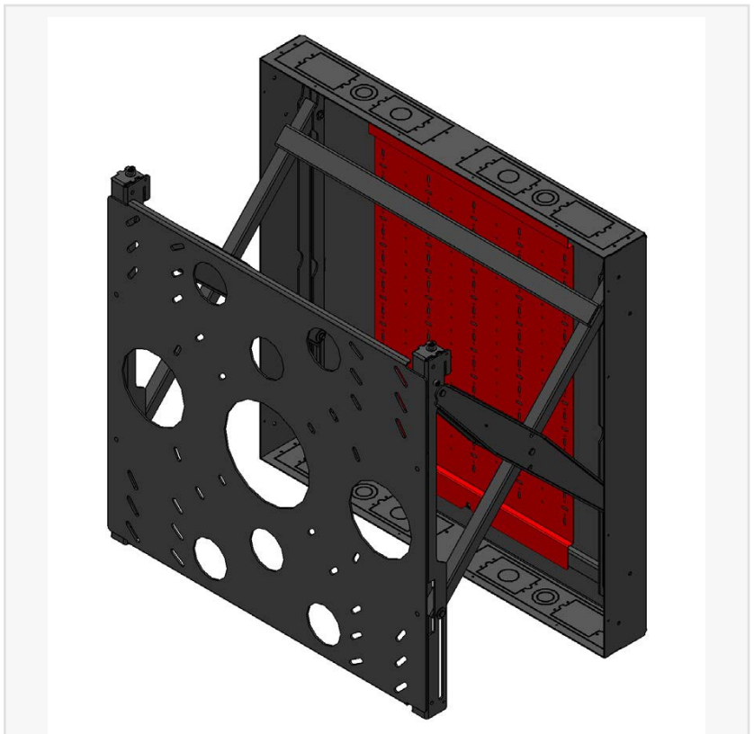
Wallmate Flush In-Wall Mounting System Helps Achieve ADA Compliance With Displays Larger Than 65" And Up To 325 lbs.
