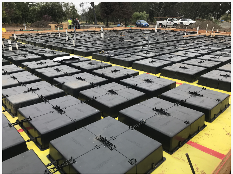
Waffle Boxes on Grade awaiting concrete to be poured for NorthStar Luxury Homes
