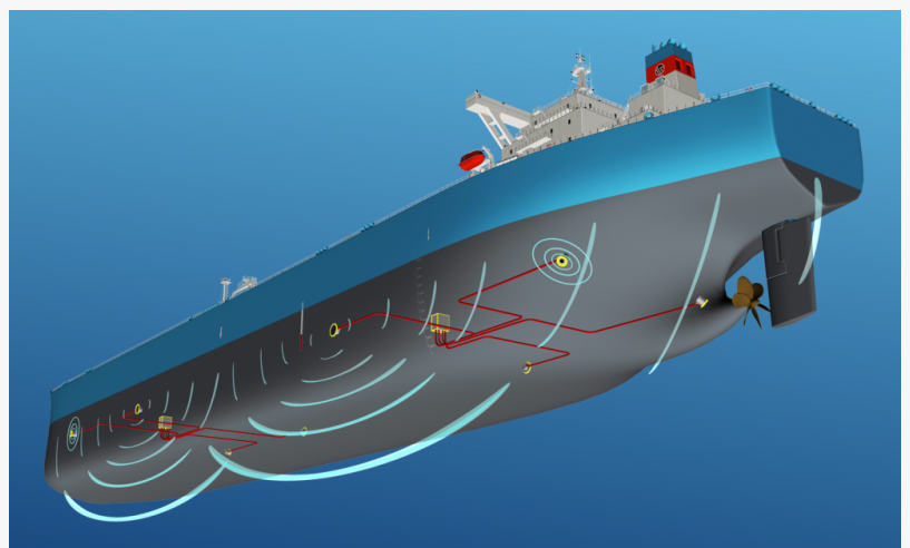
Impressed Current Cathodic Protection (ICCP) Systems
