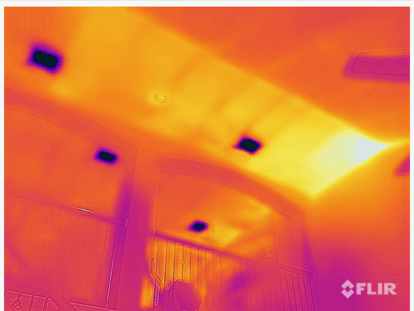
Thermal imaging photo of missing blown-in attic insulation
