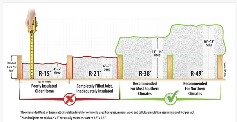
Illustration of attic floor insulation depth with R-values
