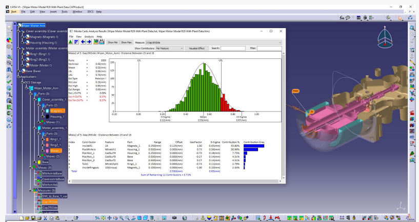
3DCS Variation Analyst Software for GD&T Creation
