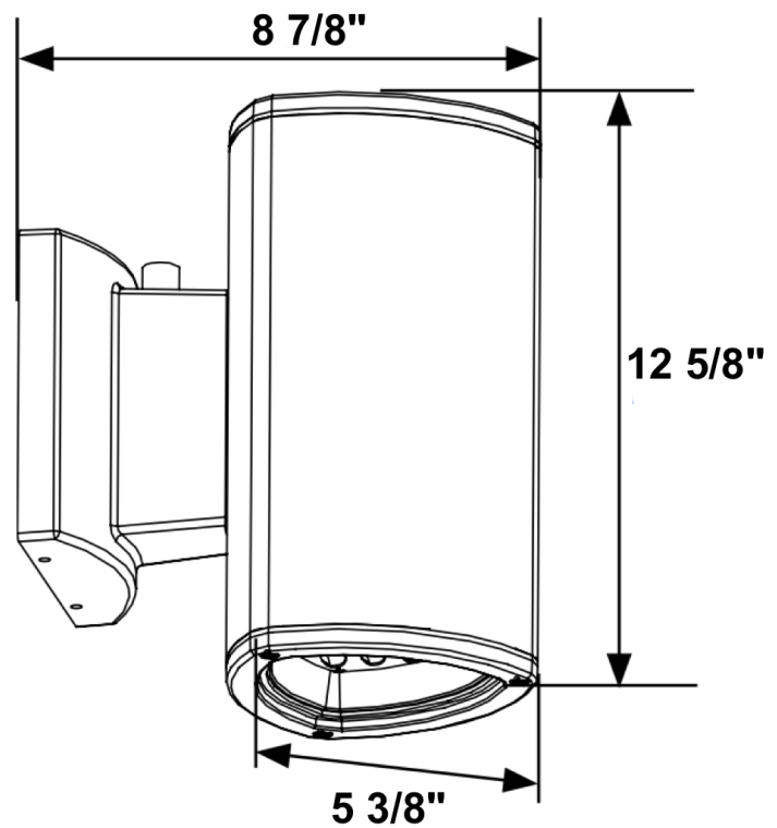
TRIS 31-watt LED Up Down Outdoor Wall Light Dimensions
