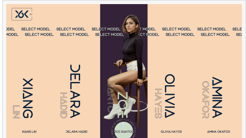
Y6K.ai website
