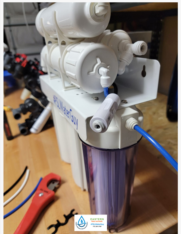
Reverse Osmosis System Installation in Port St. Lucie
