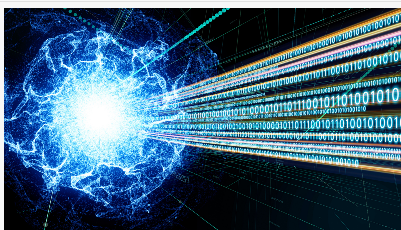
Quantum Communication
