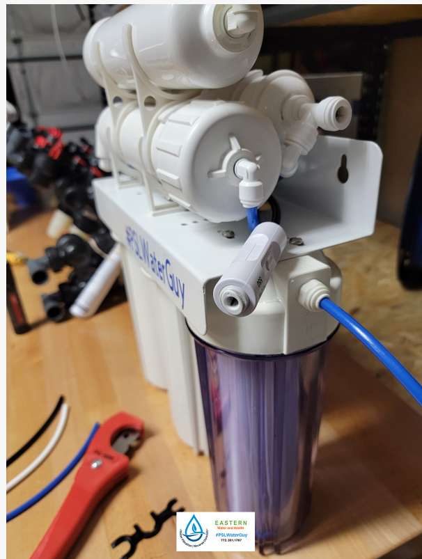
Under-the-Sink Reverse Osmosis Installation
