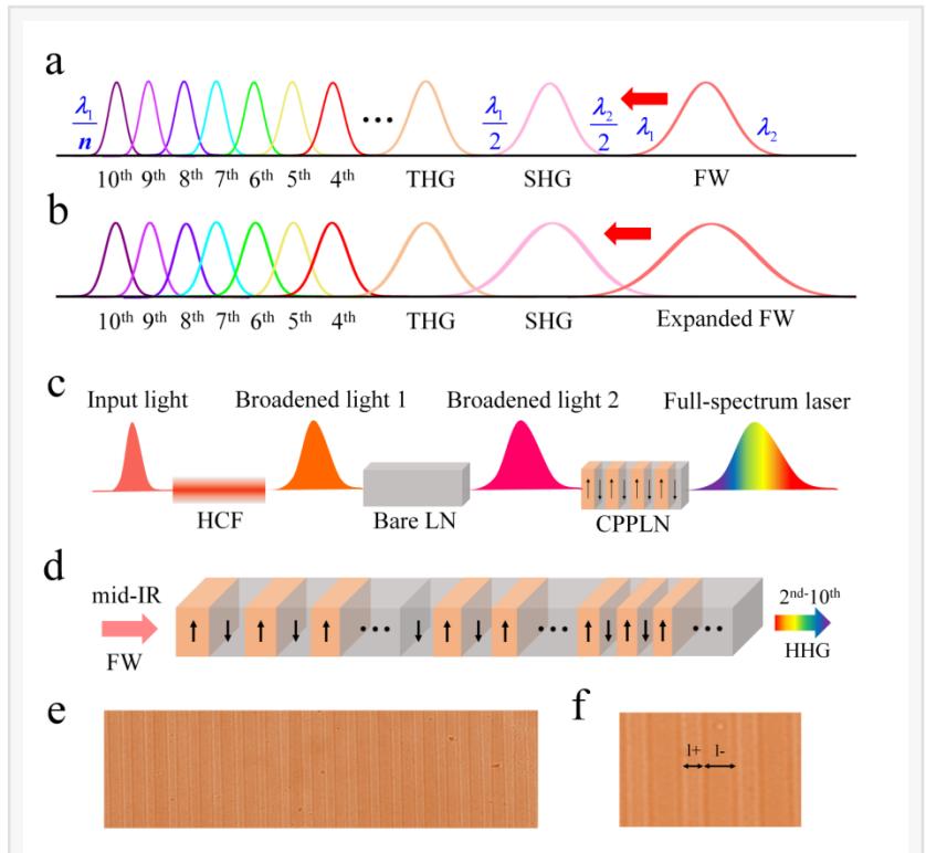
a, Schematic diagram illustrating simultaneous broadband 2nd-10th HHG via cascaded 2nd-NL QPM up-conversion upon a mid-IR pump femtosecond laser in CPPLN. b, Schematic diagram illustrating ultrabroadband 2nd-10th HHG supercontinuum white laser upon a high
