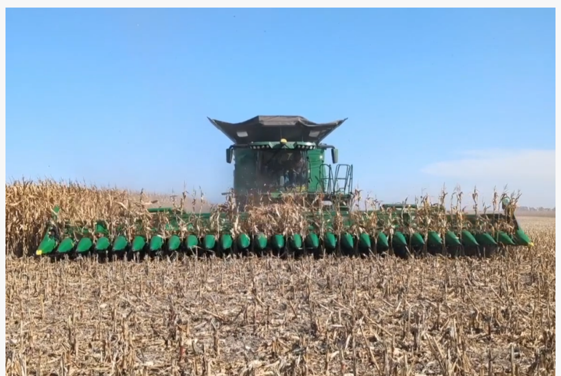
27 row 20" Corn Header, built by Bish Enterprises, harvesting corn in South Dakota
