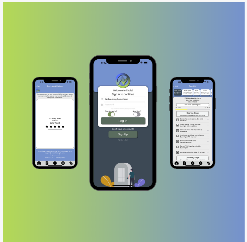
Circle Multi-screen
