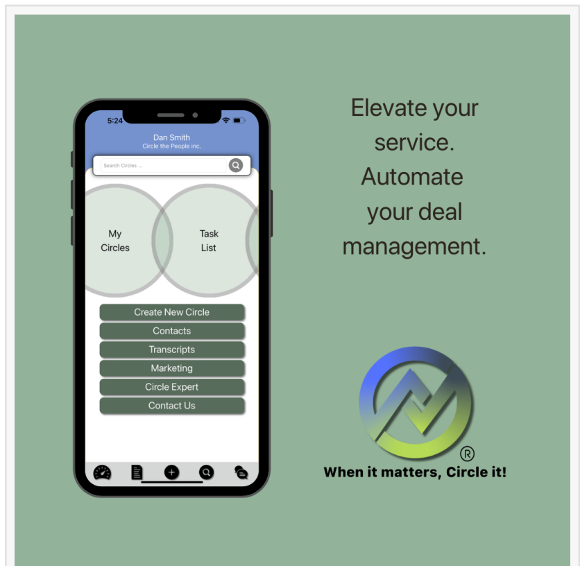
Circle Dashboard
