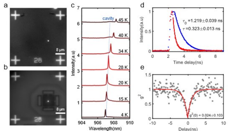
Single QD positioning and coupling to corner state.
