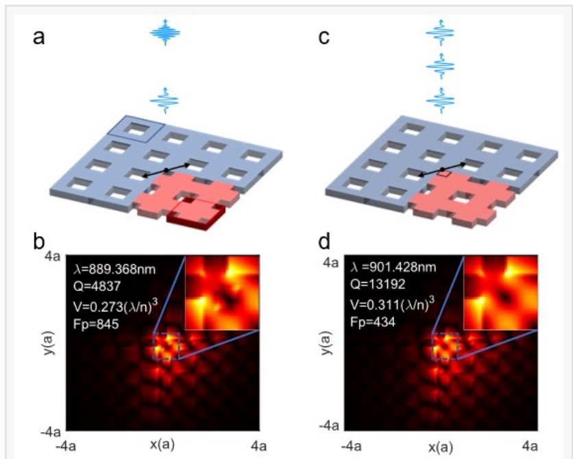
The theoretical scheme of the QD-in-topological cavity structure.
