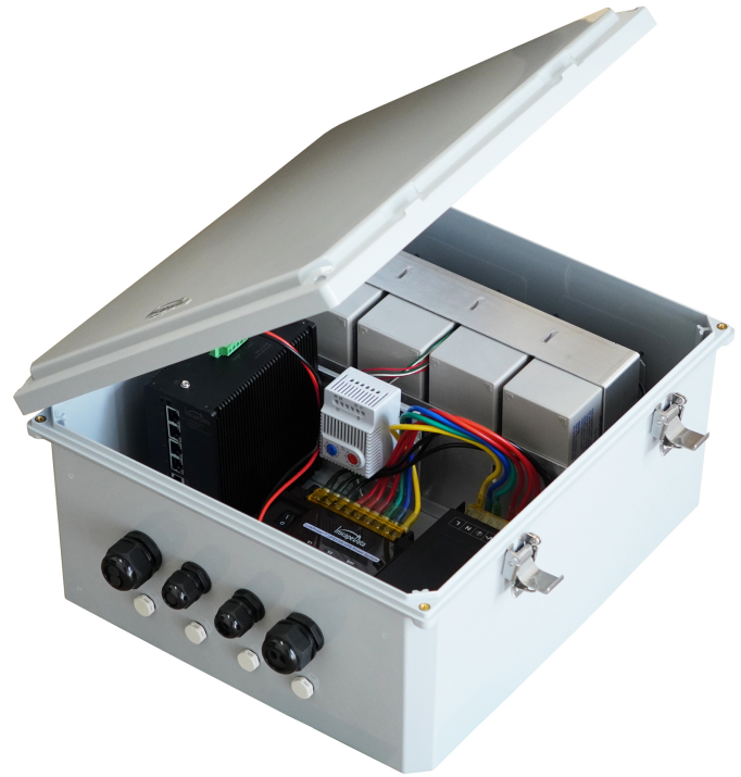
LinkPower Outdoor UPS PoE Switch System
