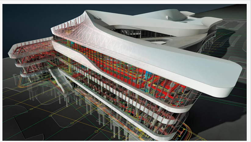
BIM Model of Architectural, Structural and MEP
