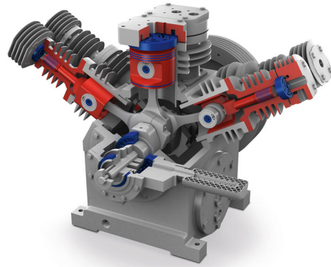
Standard High Pressure Compressor (SHP)
