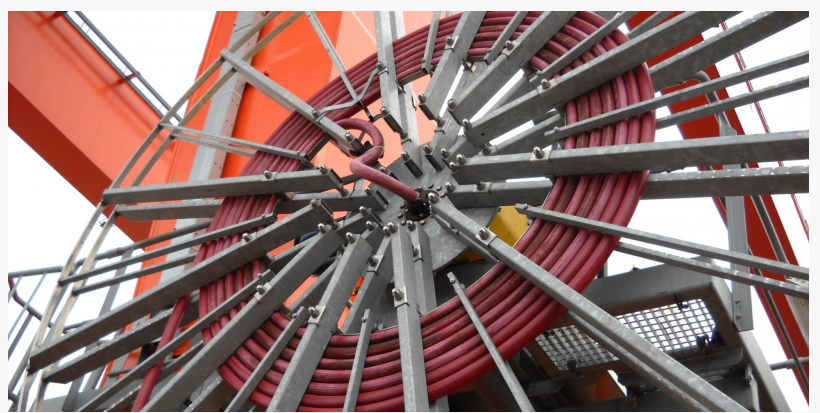
Reeling Drum Cable (600/1000V PUR sheath drum reeling cable)
