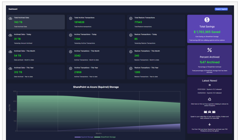
Squirrel Dashboard
