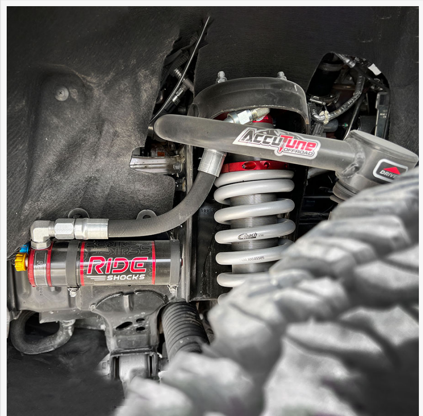
AccuTune Offroad's new Upper Control Arm paired with Ride Shocks delivers unmatched stability and extended tire clearance, designed for the toughest offroad adventures.
