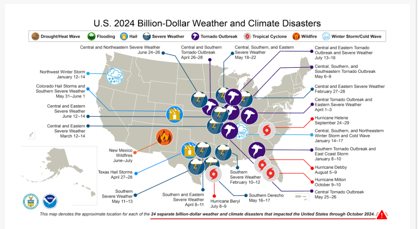
2024 United States Billion-Dollar Weather and Climate Disasters
