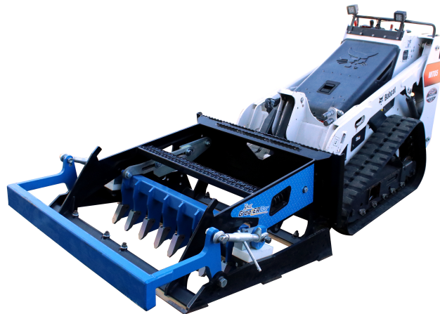
Land Plane with Rippers for Mini Track Loader
