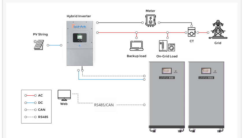
15kwh solar system connection
