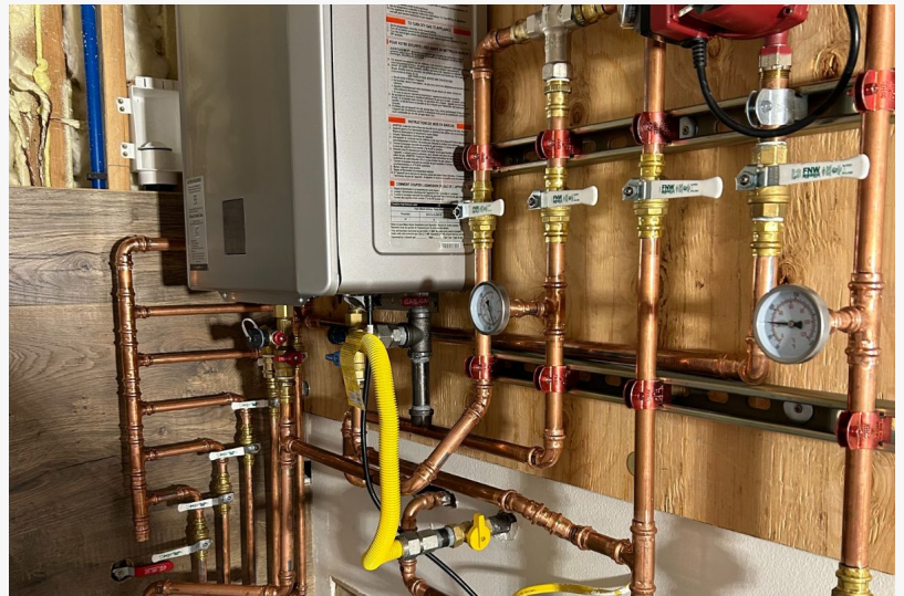
This tankless water heater installation features a custom copper piping manifold, pressure gauges, a recirculating pump, and a gas line connection, delivering on-demand hot water with maximum efficiency and reliability.
