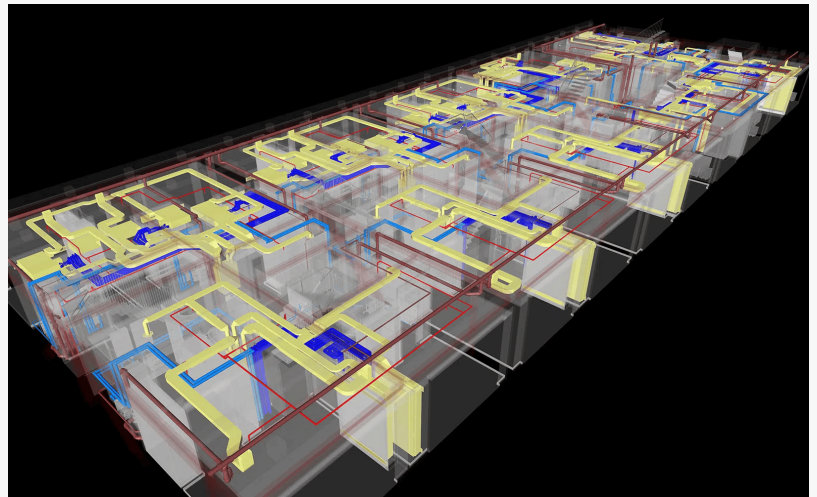
Mechanical Pipework And Fire Protection Layout - Bettersea Power Station
